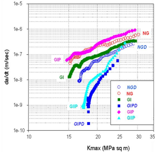
Fig. 6. Dwell fatigue crack growth rate versus maximum stress intensity for the six conditions.
