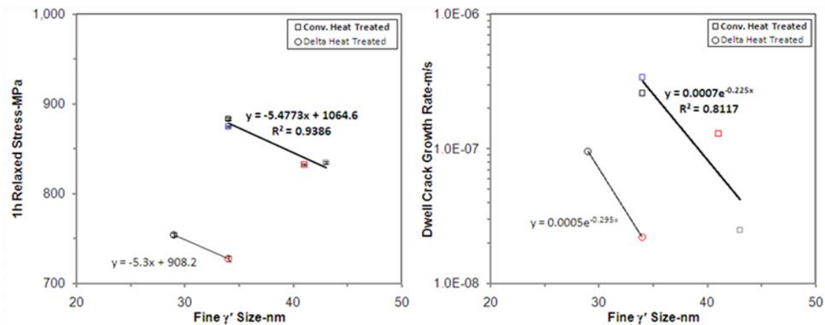
Fig. 9. Correlations of stress relaxation and dwell crack growth rate with fine \gamma' precipitate size.
