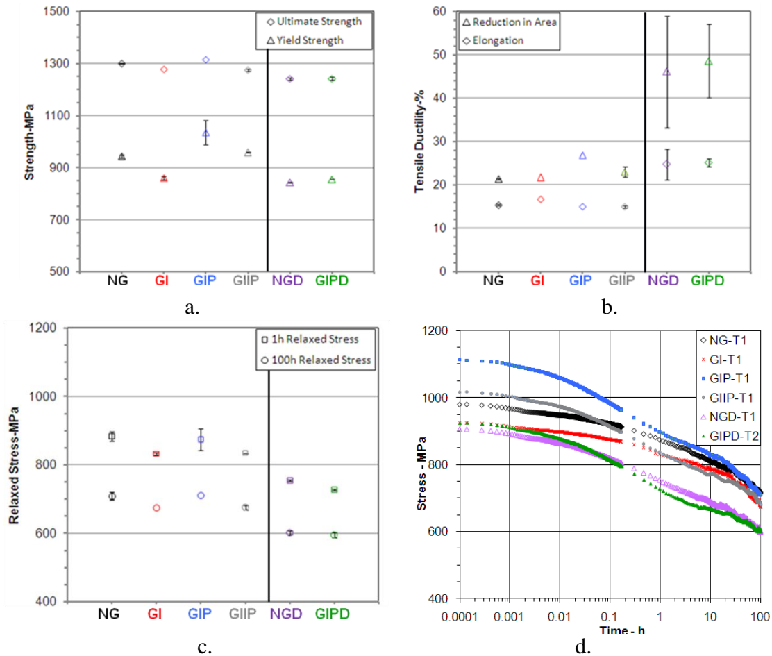
Fig. 3. Tensile response for the six conditions: a-c) mean properties, error bars indicating plus/minus one standard deviation, d) typical stress relaxation versus time.
