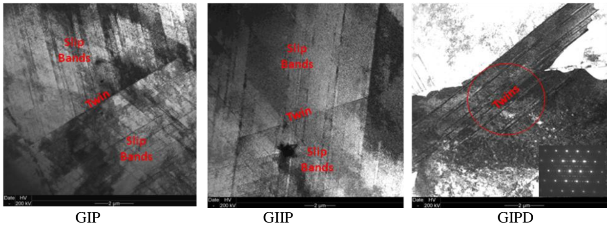
Fig. 8. Slip bands observed in TEM images of GIP and GIIP, but not GIPD material conditions.
