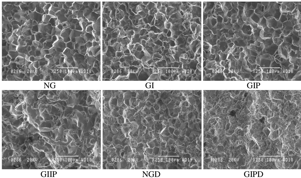
Fig. 7. Typical images of dwell fatigue crack growth regions.
