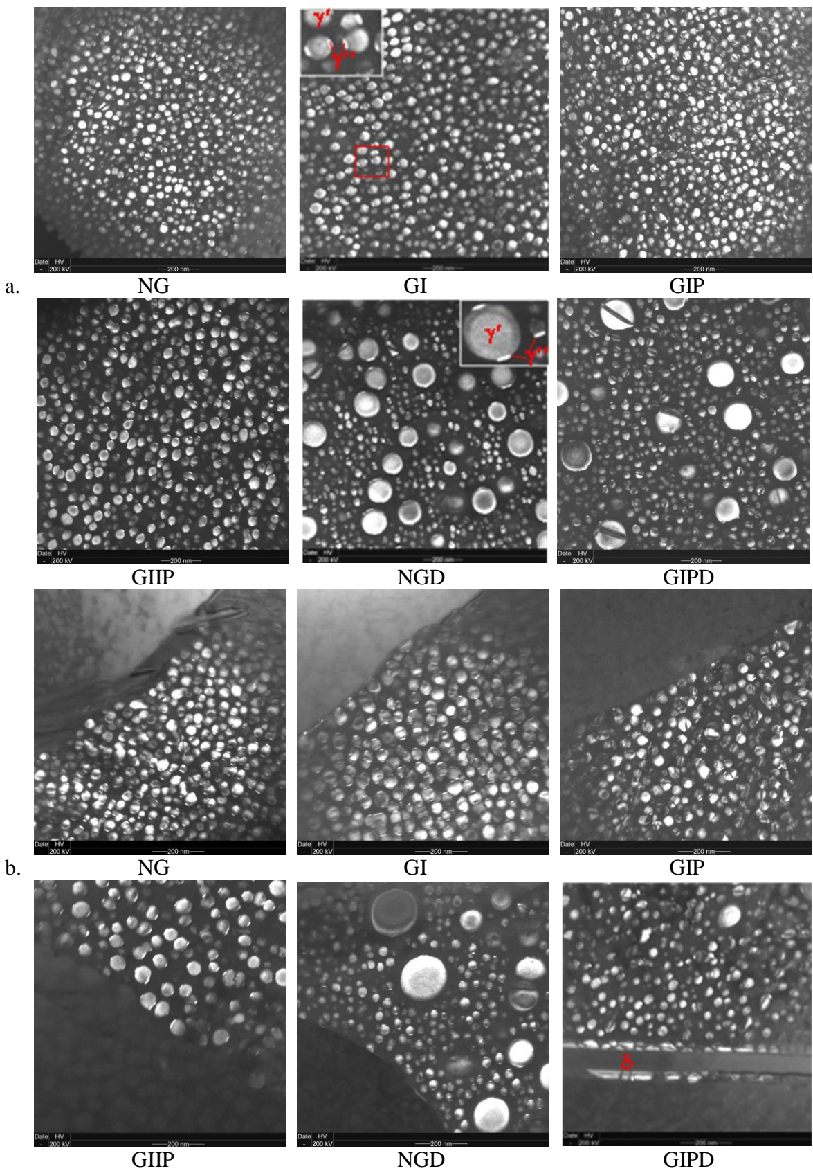
Fig. 2. TEM dark field images of \gamma' precipitates a. inside \sigma grains. b. at \sigma grain boundaries.
