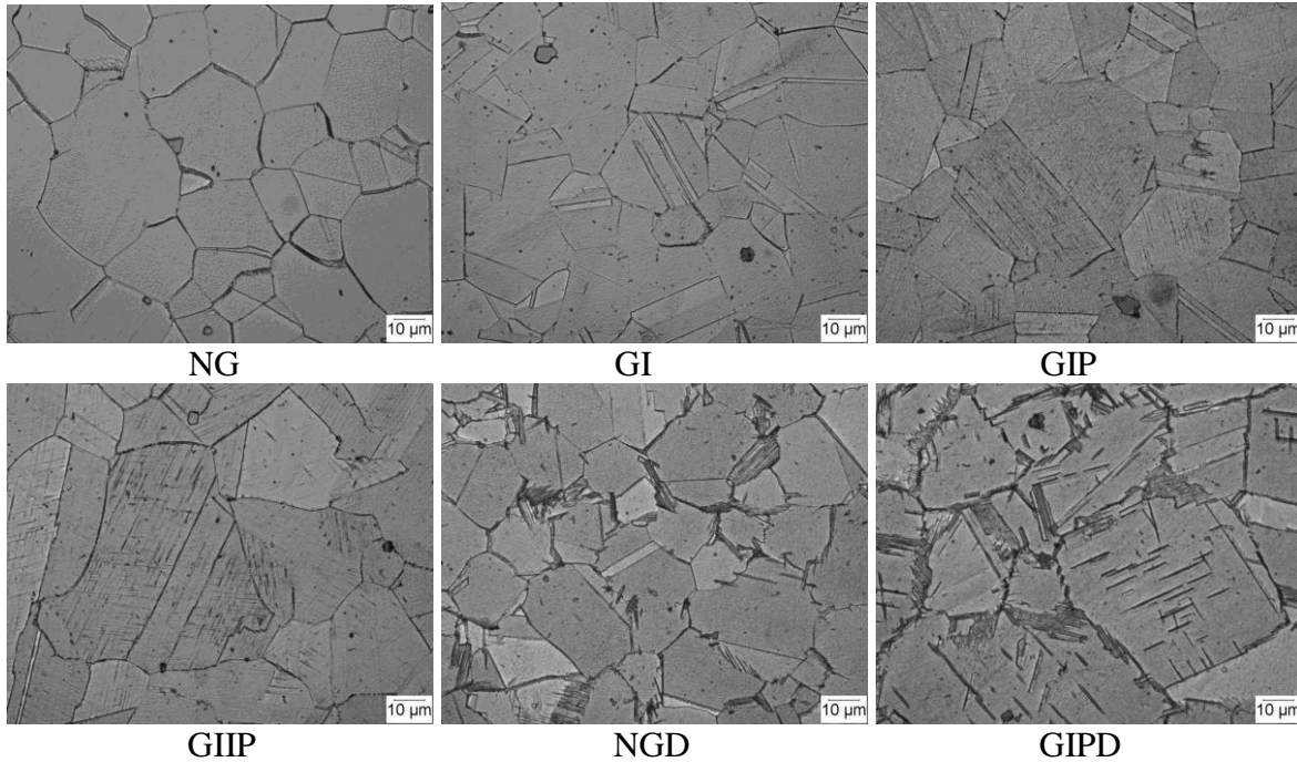
Fig. 1. Typical microstructures for the six conditions investigated.
