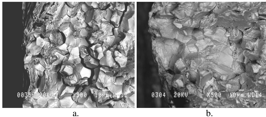
Fig. 5. Small intergranular cracks in a) NG tensile and b) GI creep failures.
