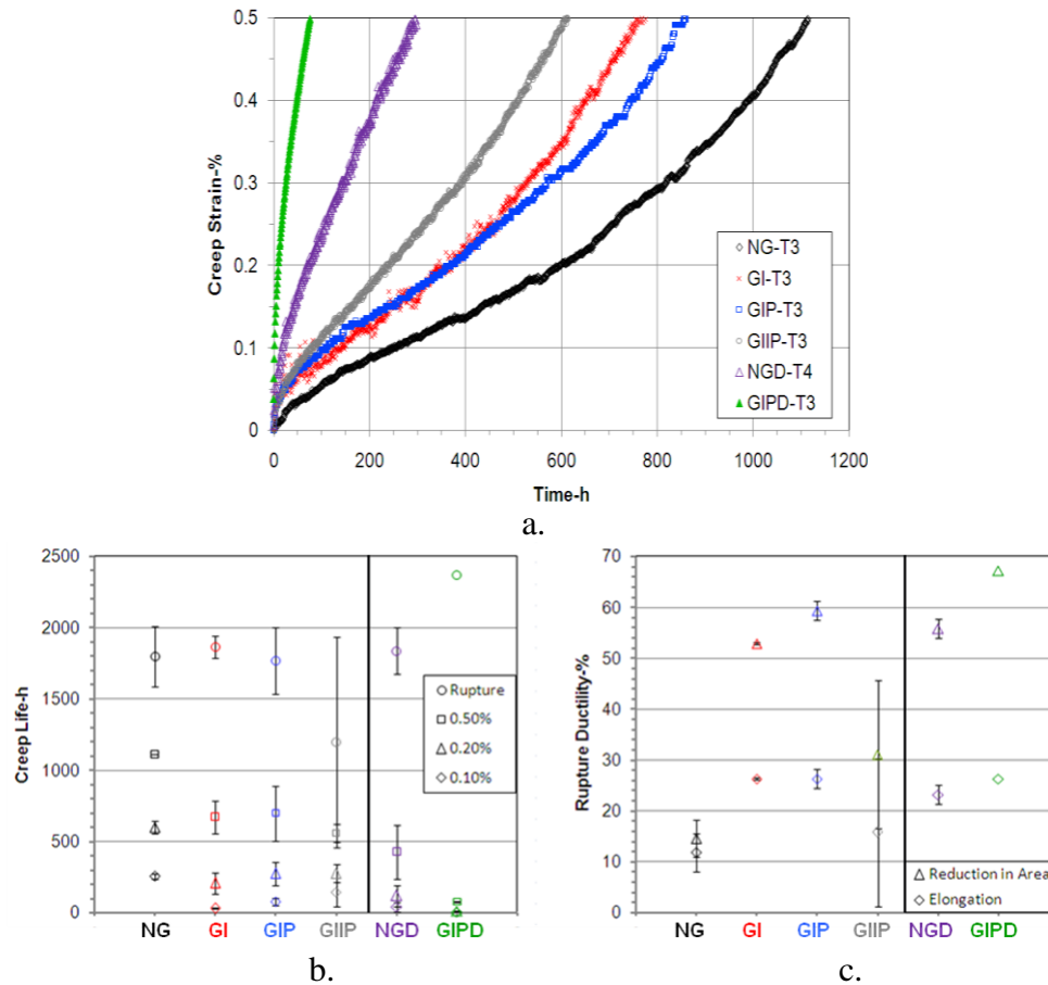
Fig. 4. Creep response at applied stress of 690MPa: a) typical creep versus time, b-c) mean properties, error bars indicating plus/minus one standard deviation for the six conditions.
